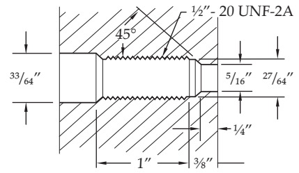
Drill Pattern
