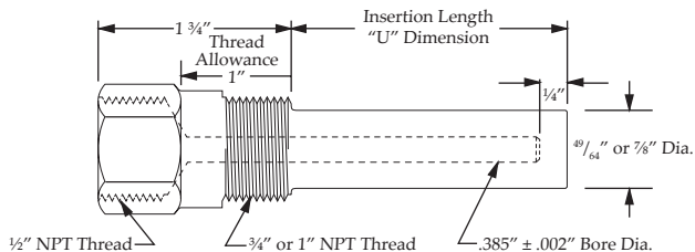
Standard Well - Straight Shank
