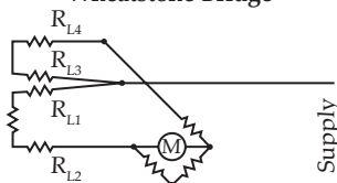
4 Wire, Compensated Wheatstone Bridge
